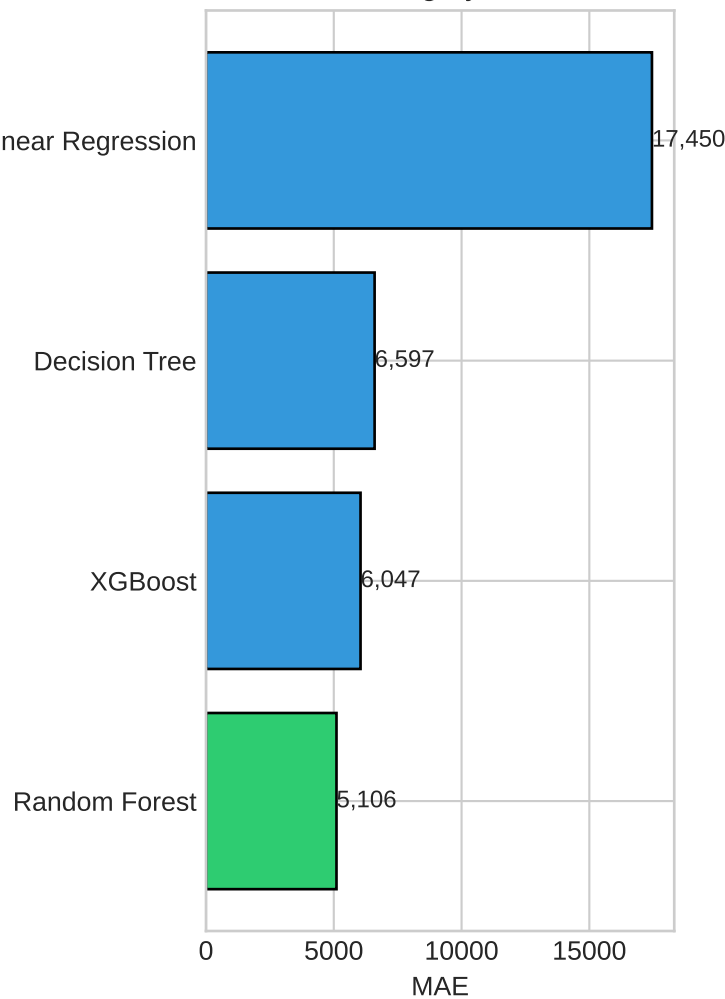
Ranking by MAE
