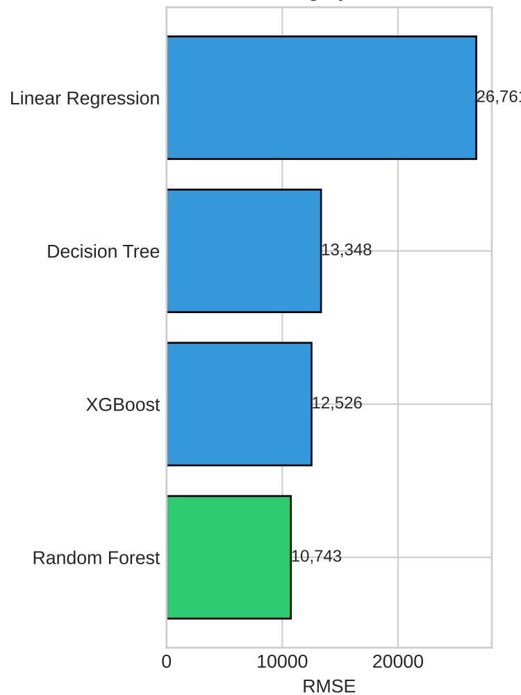
Ranking by RMSE
