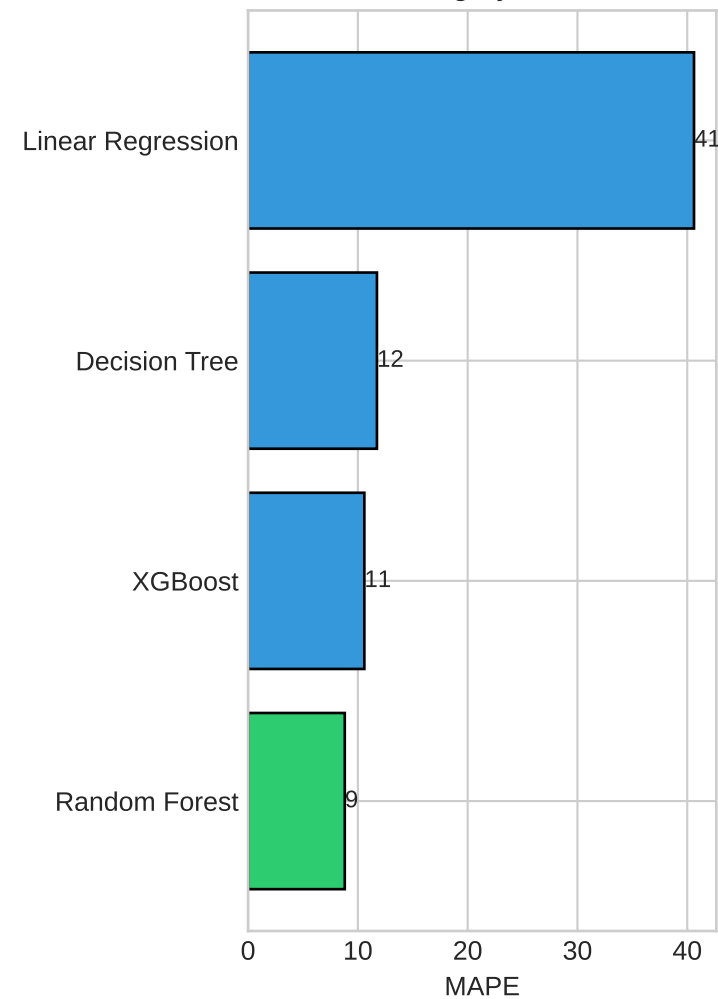
Ranking by MAPE
